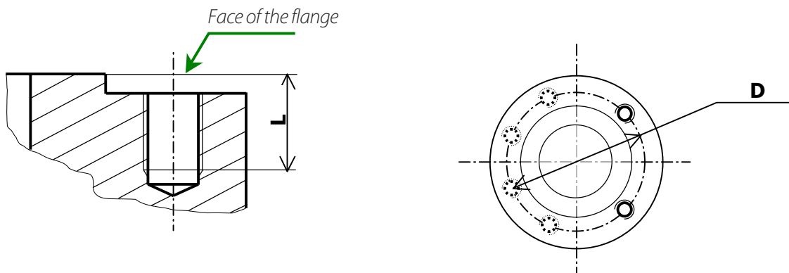
Flange meters with holes threaded
