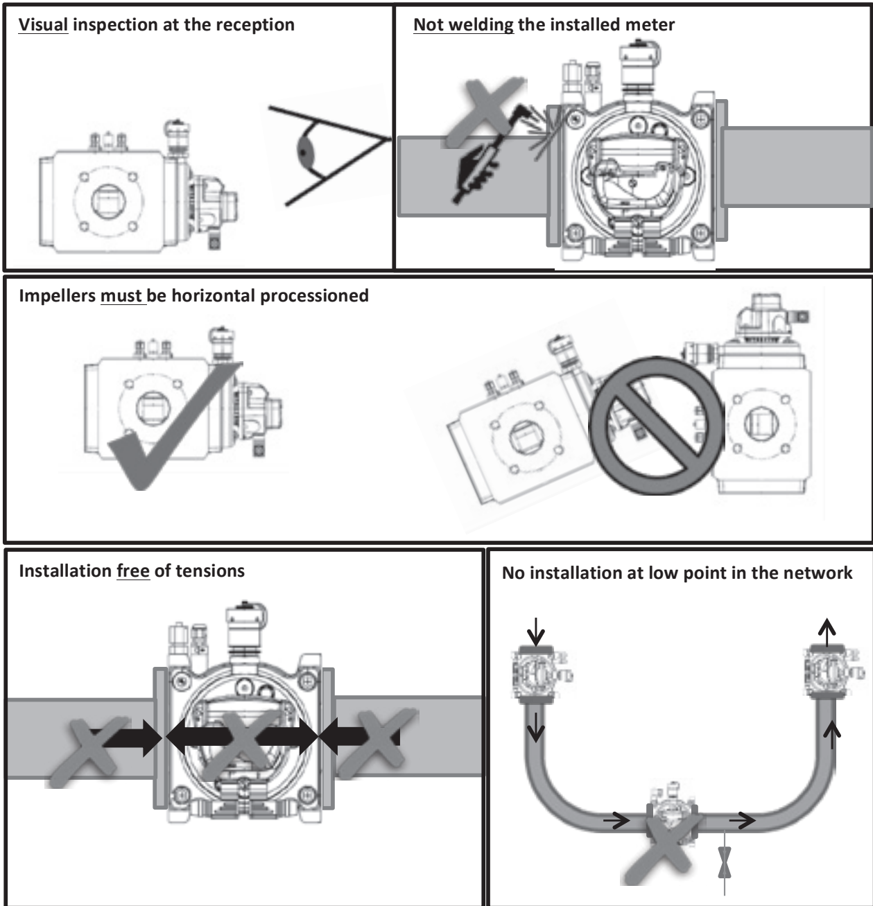
Flange meters with holes threaded
